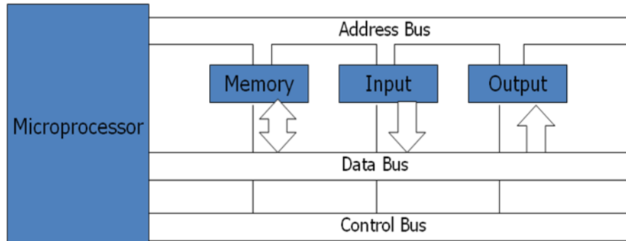
Fig: Bus Organization
